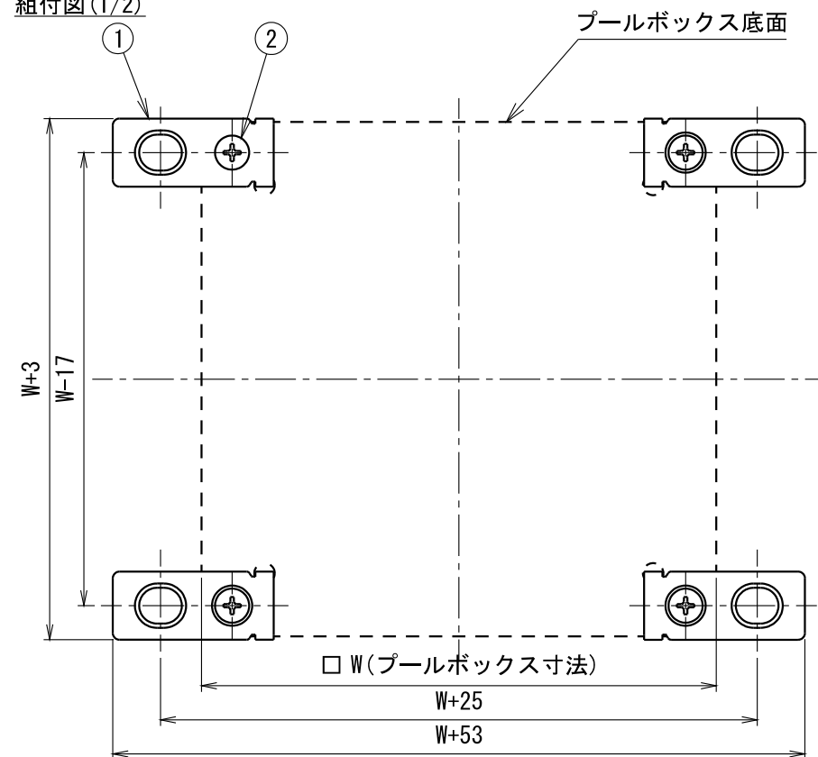
組付図(1/2)
